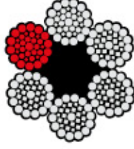
6x36 Warrington Seal
