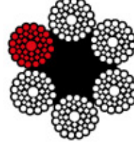
6x41 Warrington Seal
