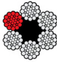
6x31 Warrington Seal
