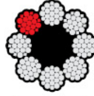
8x19 Warrington
